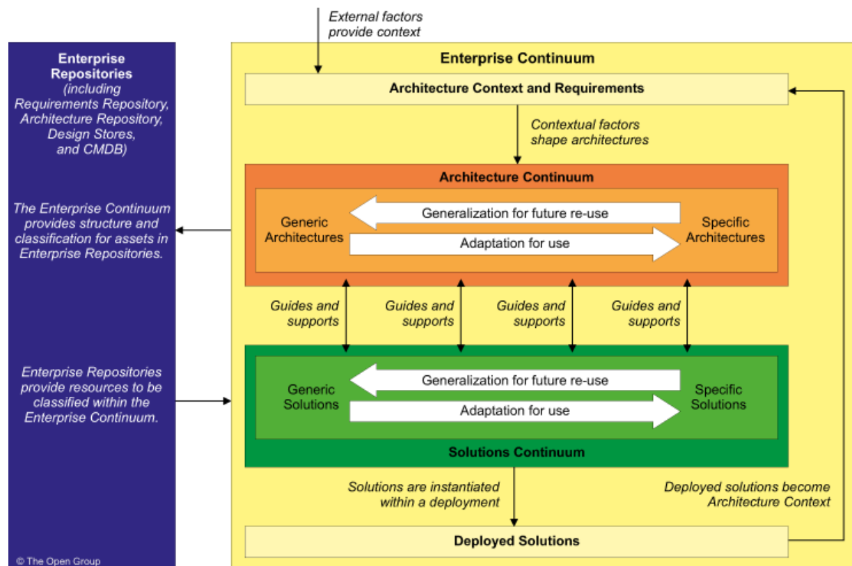
Figure 3-4 Enterprise Continuum
